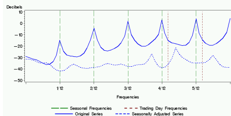
Figure 1. Example of Spectral Graph Spectrum of the Differenced Logged Original and Seasonally Adjusted Series X-12-ARIMA run of s2b3d2
